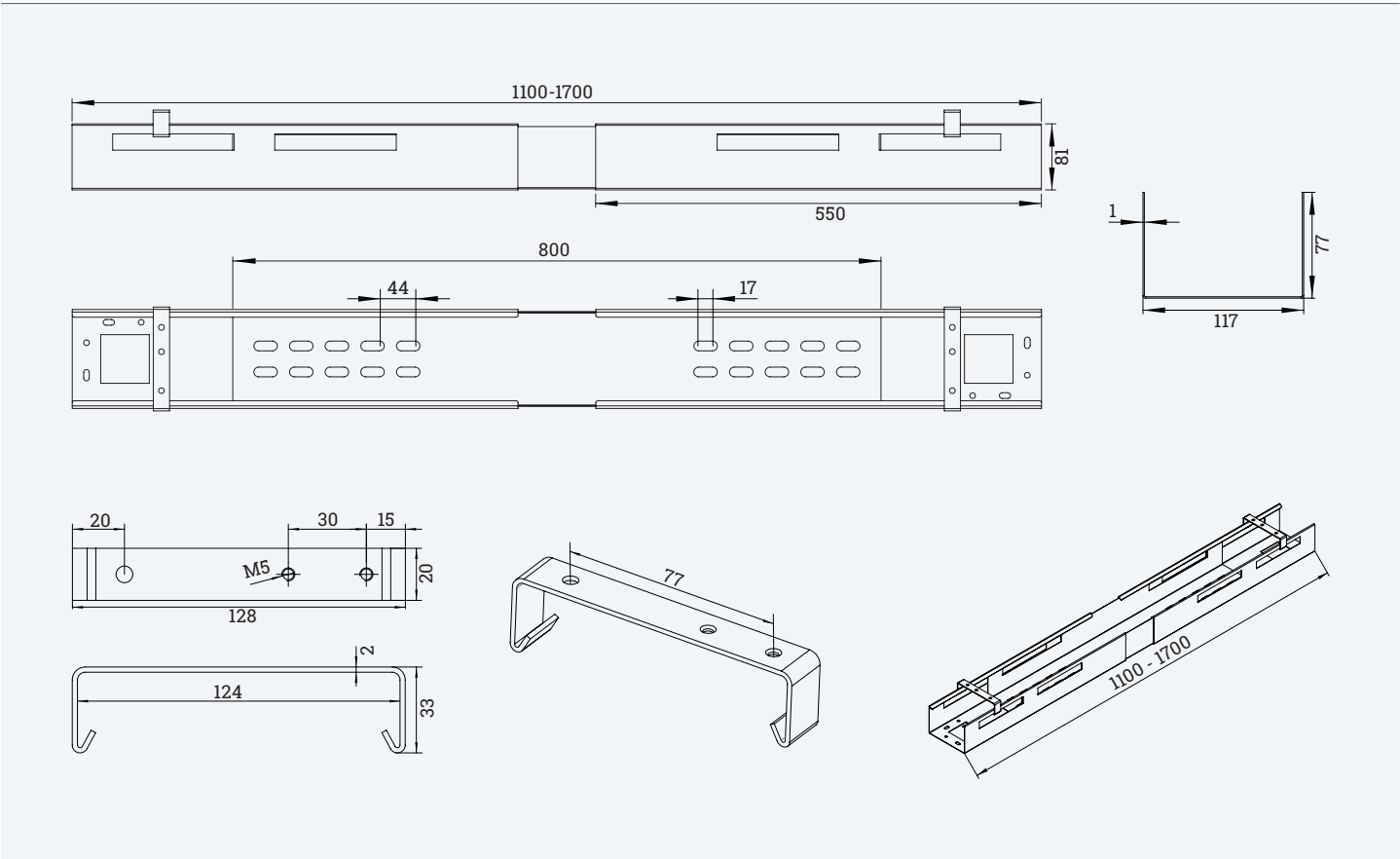
Technical drawings
