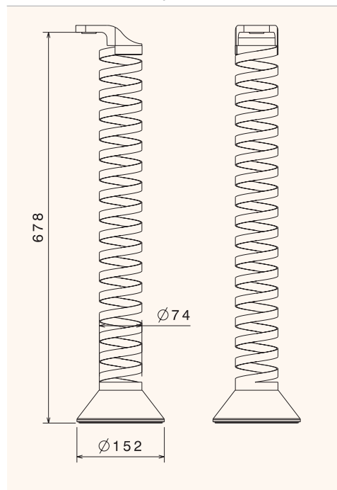
Side / Front
